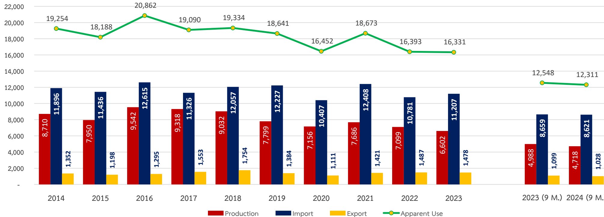
Total Apparent Finished Steel Consumption ('000 tonnes)
